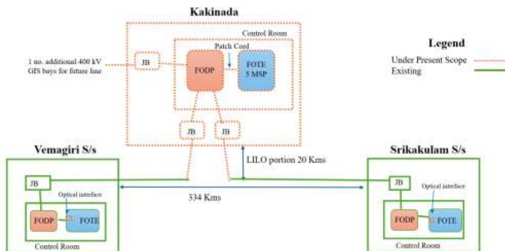
Proposed Communication for "Transmission system for Green Hydrogen / Green Ammonia Projects in Kakinada area, Andhra Pradesh (Phase-I)"
