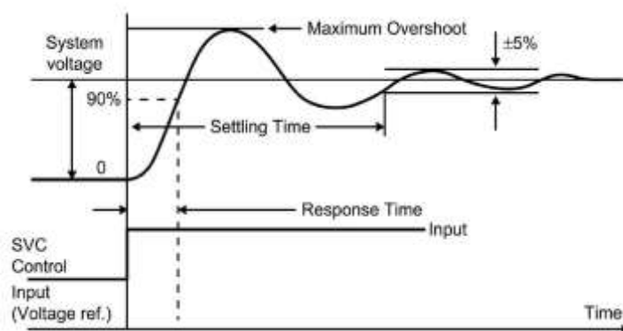
Figure-4 Response and Settling time
