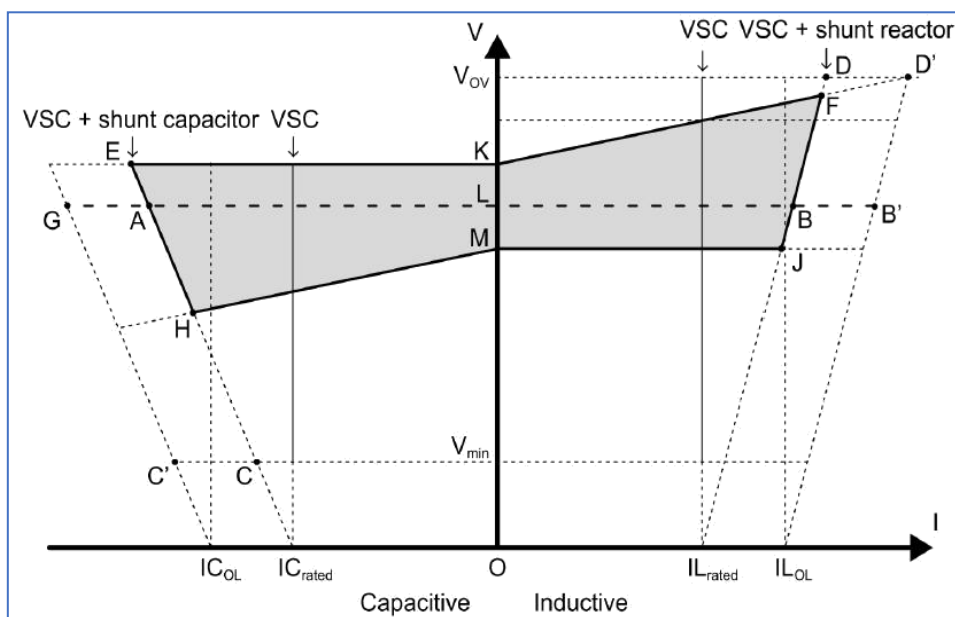
Figure-2: VI Curve of the VSC Portion
