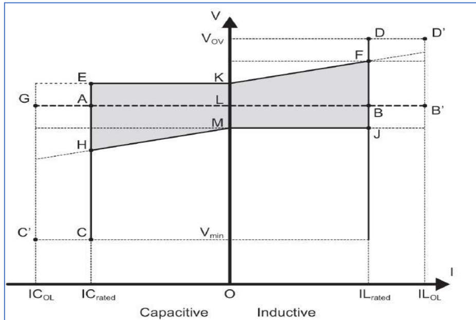
Figure-3: VI Curve of the STATCOM Station
